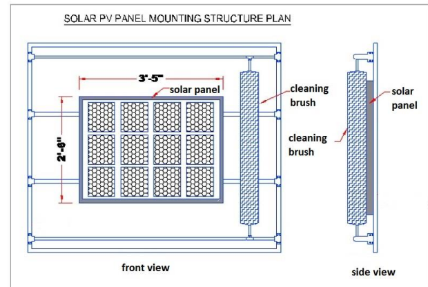
Figure.4: Mechanical structure of designed kit
